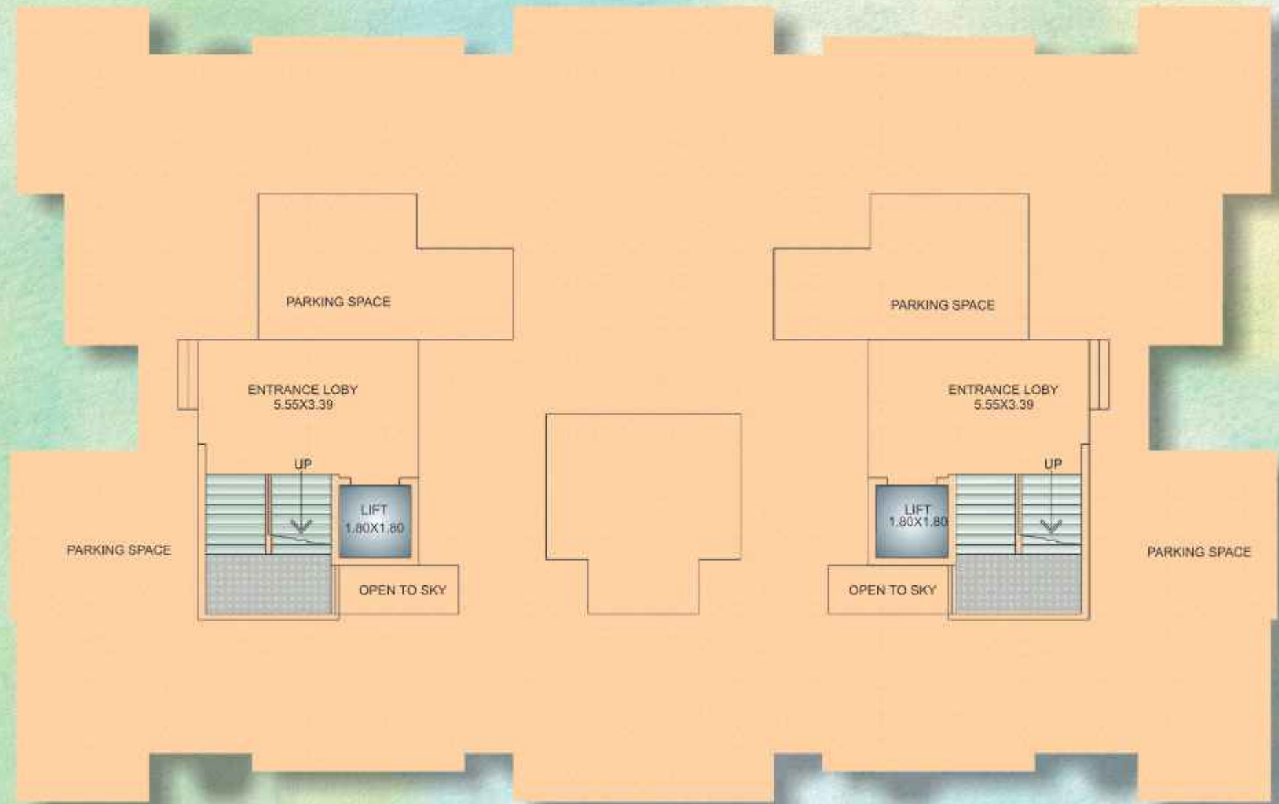
"C" WING PARKING FLOOR PLAN
